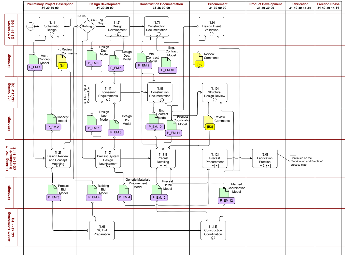
Process Map: Precaster Lead Project
