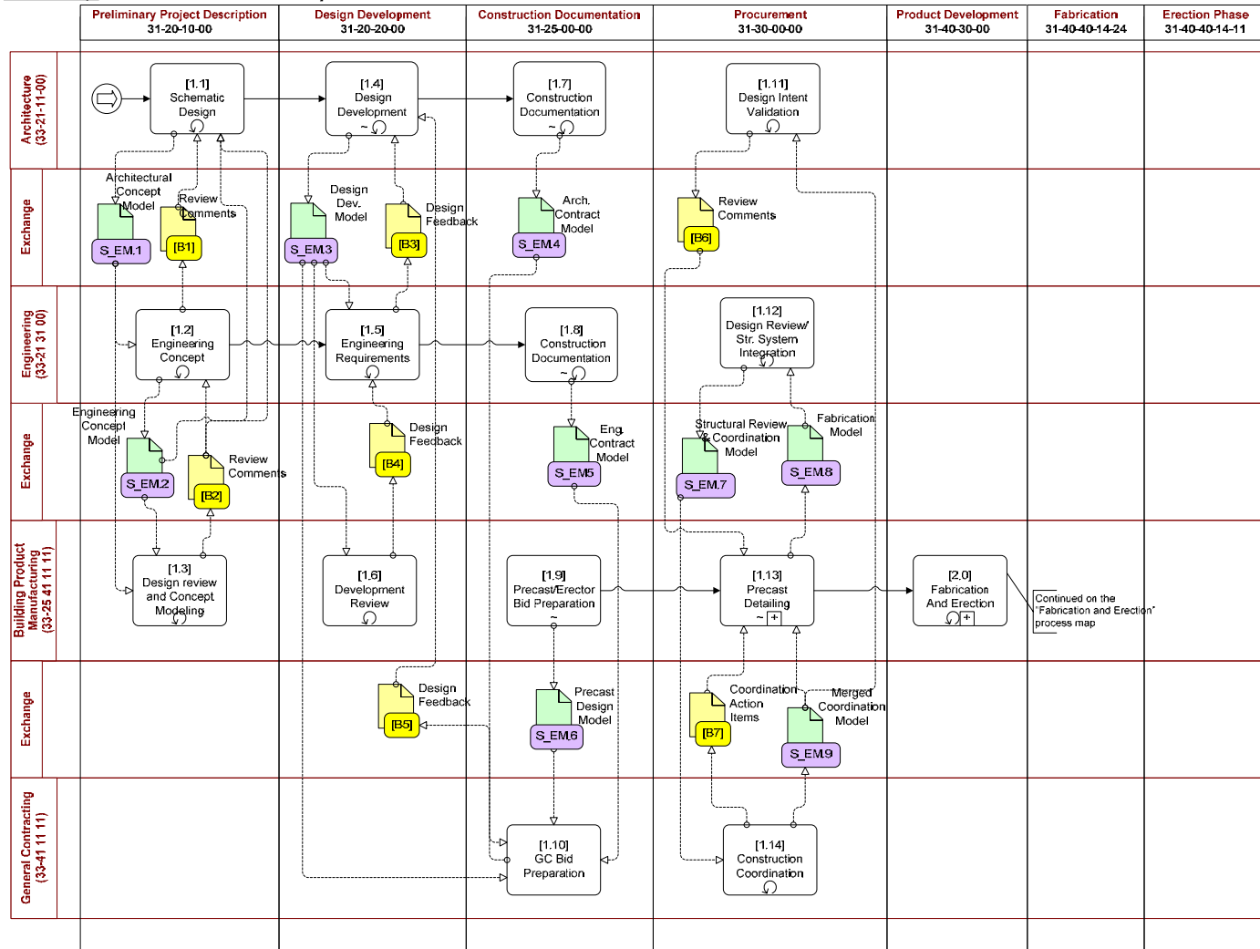
Process Map: Precaster as Subcontractor Project
