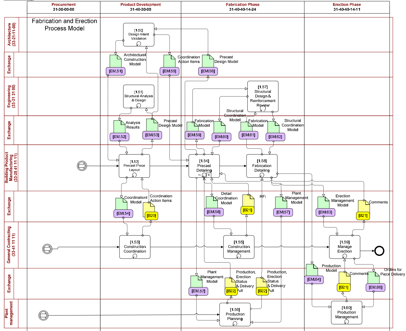
Process Map: Fabrication & Erection
